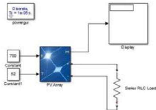
Figure 1. Photovoltaic modeling via Matlab/Simulink
