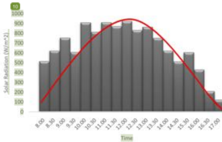
Figure 4. Graph of solar radiation absorption at a slope of the angle of 50°
