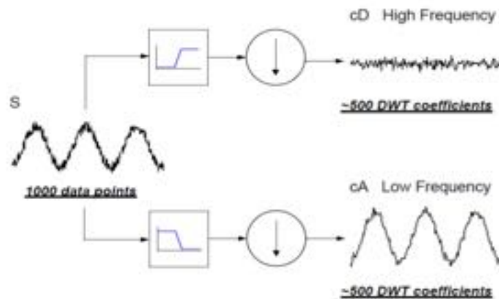
Fig. 1. Diagram signal processing DWT
