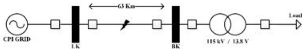
Fig. 4. Single line diagram transmission system
