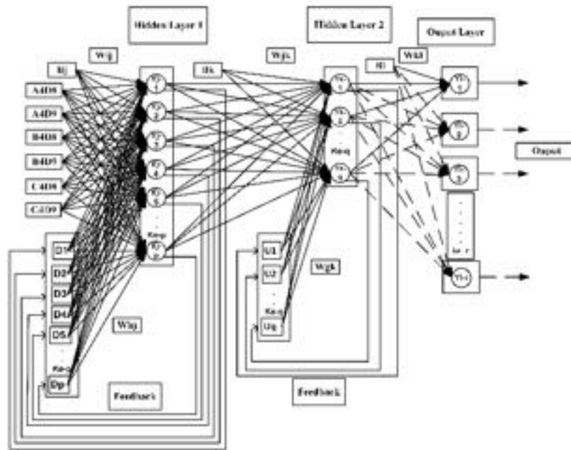
Figure 6. Elman RNN structure estimated fault location
