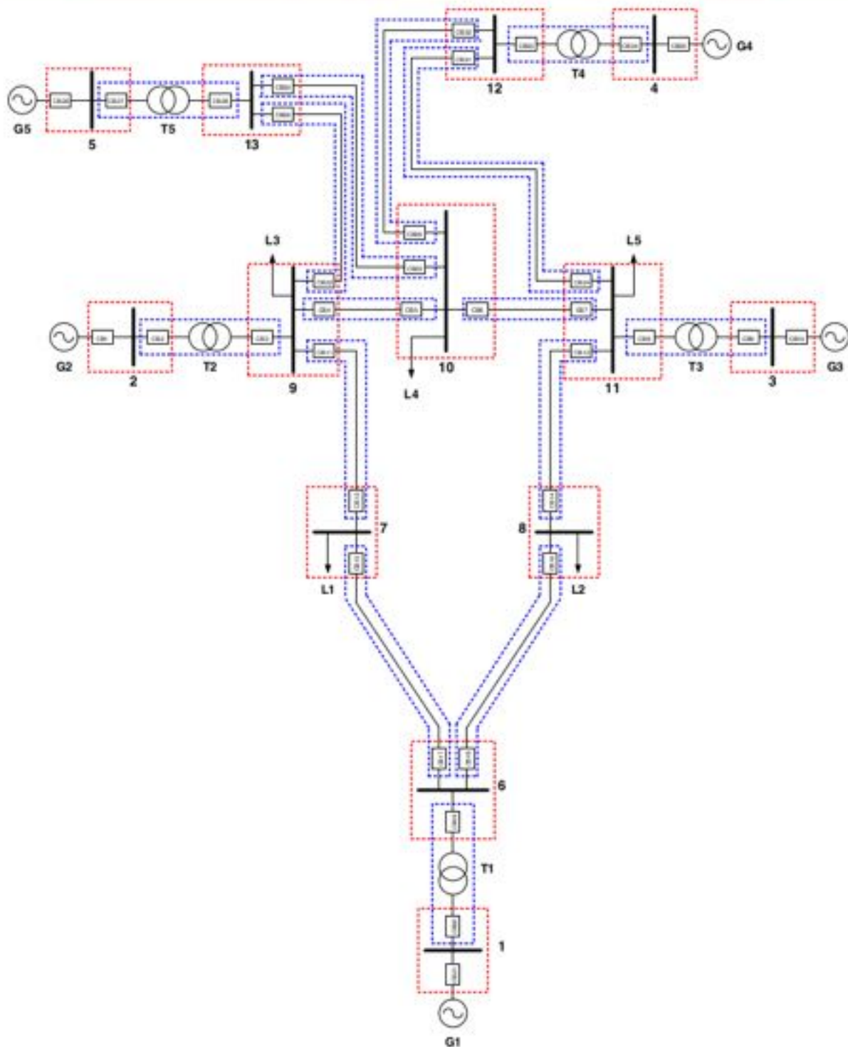
Fig. 3. The 13 bus system protection
