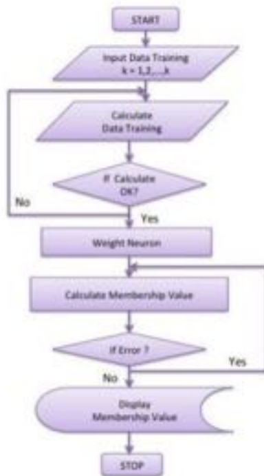
Fig. 4. Flowchart to generate membership value
